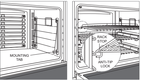
Oven rack guide Oven rack anti-tip lock
